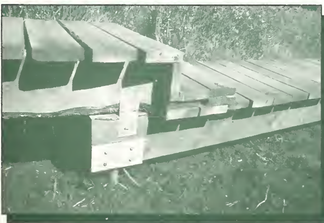
Figure 38—A helical pile was used for this boardwalk. Stringers are attached directly to the beam saddle, helping to keep the boardwalk close to the ground.
